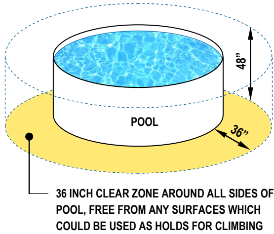
ABOVE-GROUND POOL WITH POOL WALL AS BARRIER
